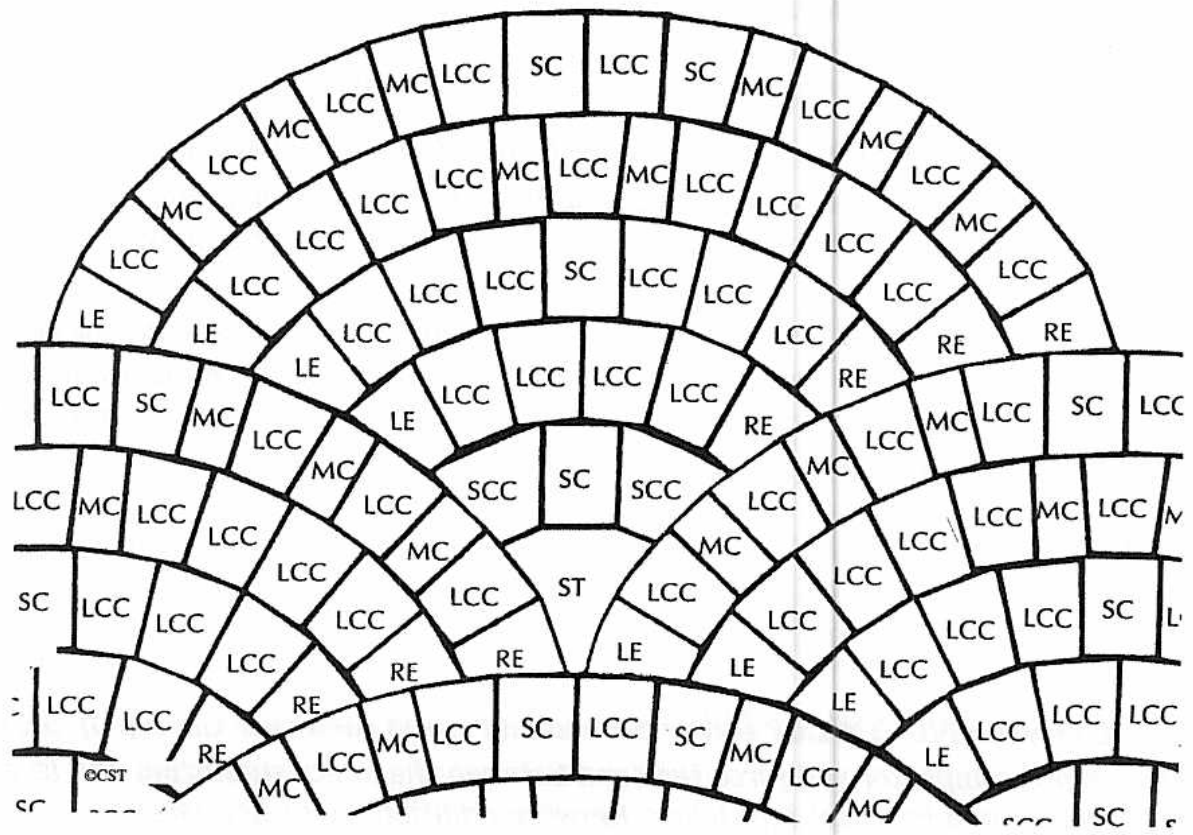
Roman Cobble® Fishscale® Layout
